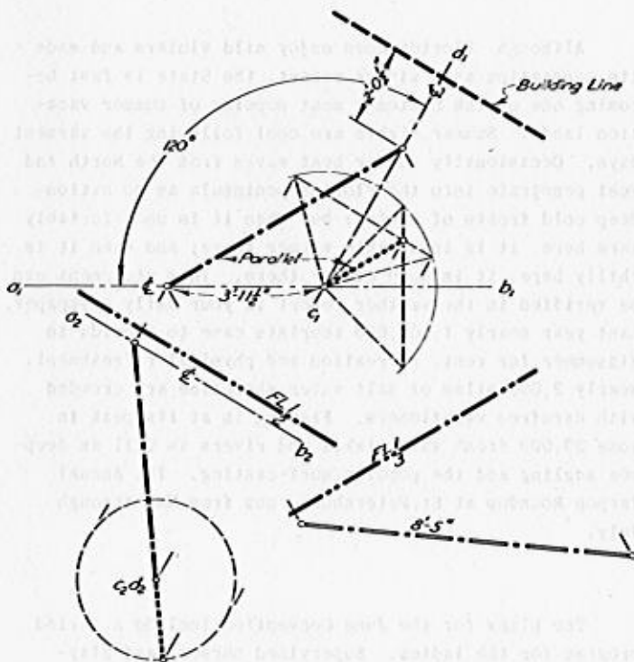
Fig. 1 (Graphical Solution)
