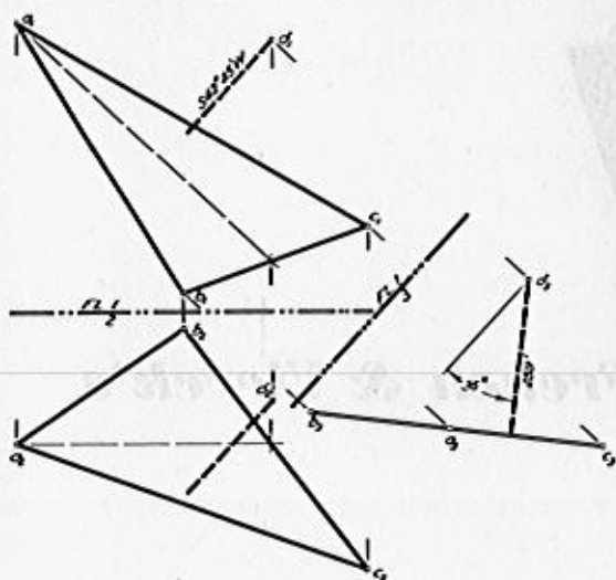
Fig. 3 (Graphical Solution)
