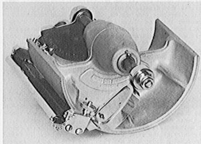
A Dermatome
