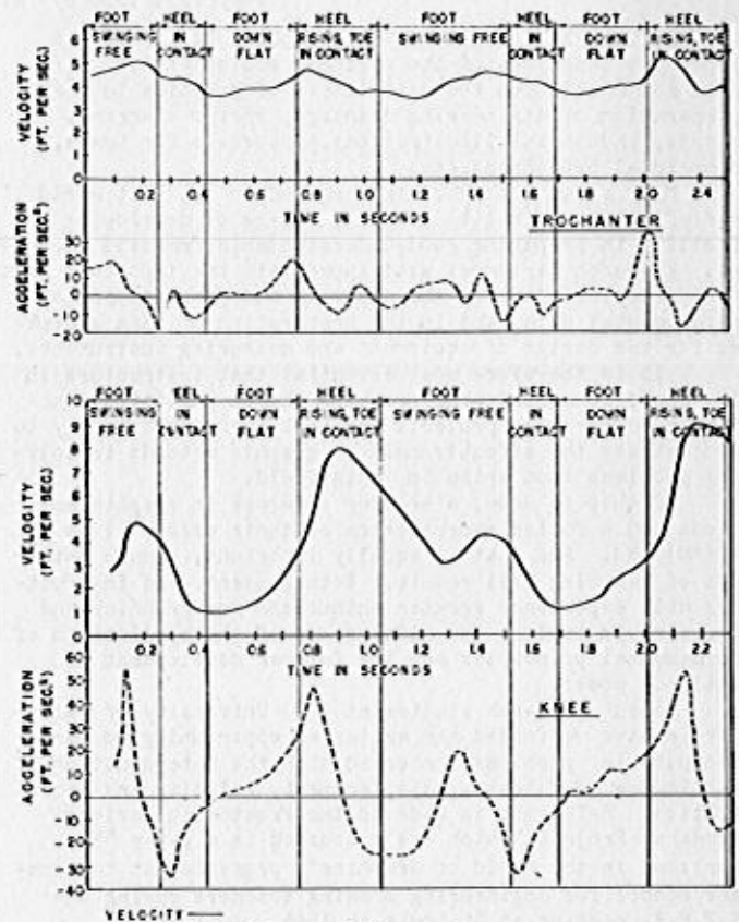
Figure 3 Horizontal Velocity and Acceleration of joints of the leg - normal level walking.
