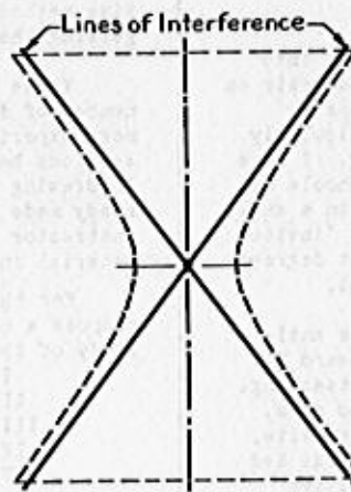
Fig. 2 Hyperboloid generated. Lines of interference appear as asymptotes of the hyperbolic outline.
