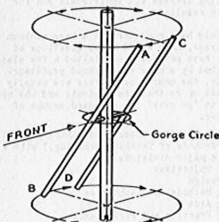
Fig. 1 Rods AB & CD, 180° apart at gorge circle, are for the first and second generation.
