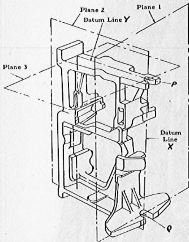
Figure 4 Pictorial view included as a part of the shop drawing of the Step-by-Step switch frame as die cast from aluminum alloy.
