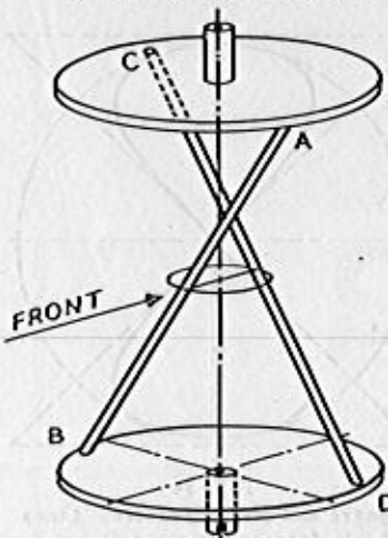
Fig. 5 Rods AB & CD, 180° apart at gorge circle, are for the same generation.
