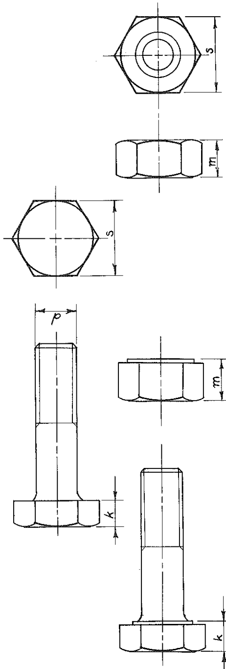
1. BASIC DIMENSIONS: METRIC SYSTEM
