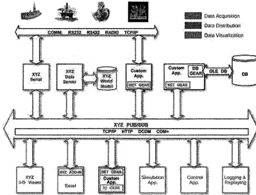
Figure 4. XYZ-Solutions Architecture.
