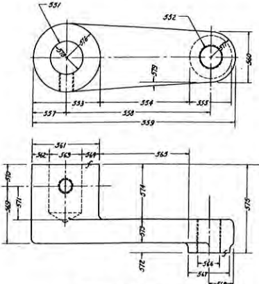
THROW-LEVER LINK
