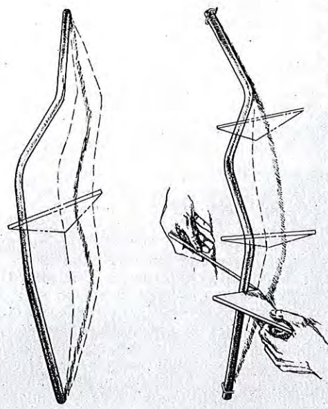
Fig. 3. One of the many mechanical aids used to obtain information on certain technical sketches is illustrated in the method of recording the shape of a tube used in the installation in the airplane. The tube is secured to the fuselage on one side, the base of the triangle resting flat on the sketch paper. Small dashes are drawn at the base of the triangle as it is gradually moved along the length of the tube (bottom figure). A second orthographic view of the tube is drawn (top figure). To represent the outside edge of the tube, the acquired lines of course are added. The diameter and centerlines are added.
